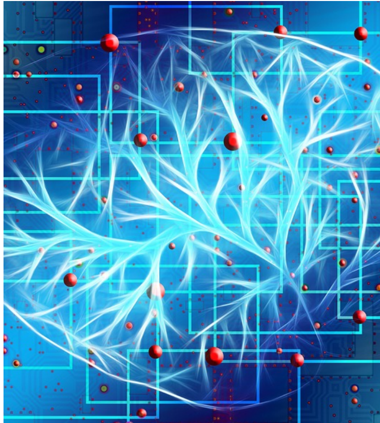
Artificial Intelligence
