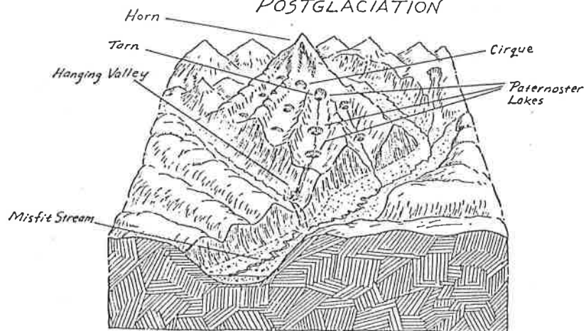
Topographic modification by Alpine glaciation
