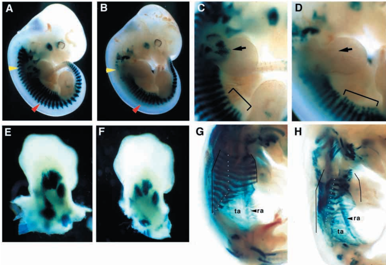
Fig. 2. Formation of hypaxial muscles is delayed in the paraxis -/- embryos. Expression of the myogenin-lacZ transgene was visualized by X-gal staining in E11.5 (A-D), E12.5 (E,F) and E13.5 (G,H). At E11.5, the myotome and primordia for migratory muscles in the face, forelimb and hindlimb express the myogenin-lacZ transgene in wild-type embryos (A,C). In paraxis -/- embryos (B,D), the medial myotome is truncated (red arrowhead) and ventral tips of the myotome are bifurcated (bracketed). The primordia for the appendicular migratory muscles are absent in the E11.5 paraxis -/- embryos, pectoral girdle (yellow arrowhead) and forelimb (black arrow). Myogenin-lacZ -positive cells are present in the forelimbs of both wild-type (E) and paraxis -/- (F) embryos at E12.5. In E13.5 wild-type embryos (G), the intercostal muscles have migrated ventrally in a differential manner that reflects the shape of the adjacent developing rib. The corresponding intercostals (white dots) in the paraxis -/- embryos (H) fail to migrate ventrally to the same extent. Ra, rectus abdominus; ta, transverse abdominus
